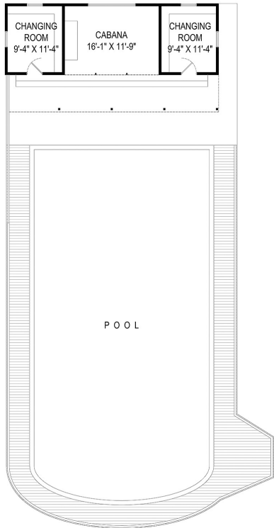
POOL HOUSE FLOOR PLAN 446 SF
