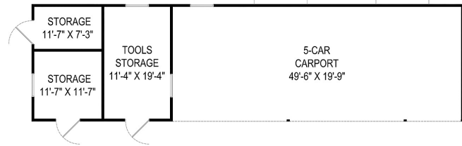
CARPORT & STORAGE FLOOR PLAN
